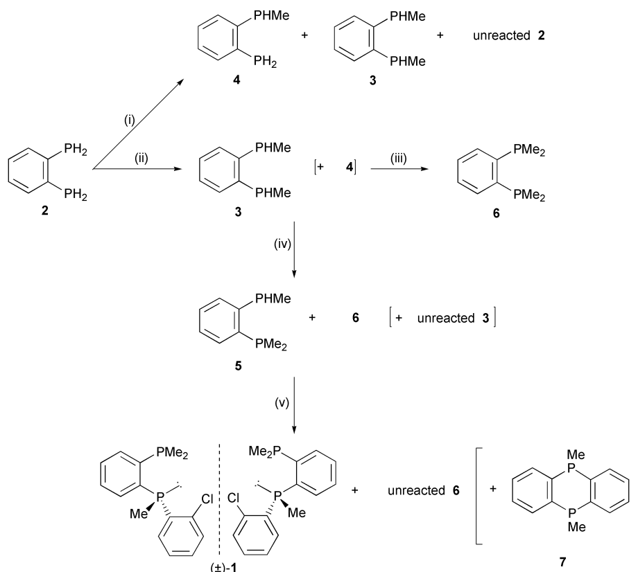
Scheme 1 (i) Na in THF; MeI; (ii) 2 Na in THF; MeI; (iii) 2 Na in THF; MeI; (iv) 1.2 equivalent K in NH 3 (l); MeI; (v) Na in THF; 1,2-C 6 H 4 Cl 2 .
