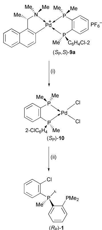
Scheme 3 (i) Concentrated \text{H}_2\text{SO}_4 ; ice, LiCl; (ii) \text{CH}_2\text{Cl}_2 ; KCN in water.
