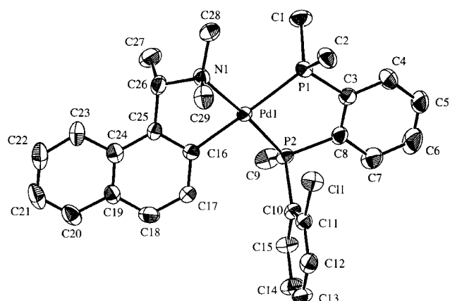
Fig. 1 Molecular structure of the cation of complex ( S p ,S )- 9a . (The thermal ellipsoids show 30% probability levels.)
