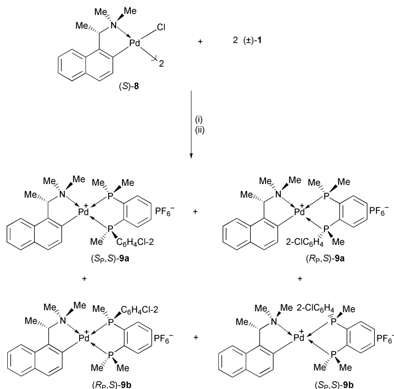
Scheme 2 (i) MeOH; (ii) \text{NH}_4[\text{PF}_6] in water.
